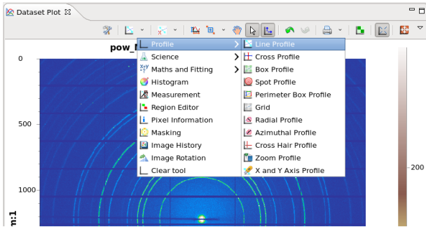
Figure 2: Some of the available tools for 2D data
