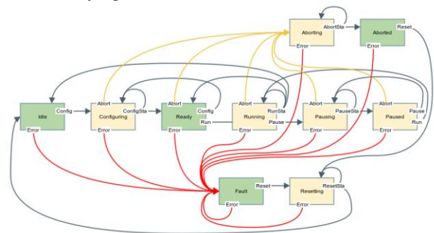
Figure 3: Design of Malcolm state machine
