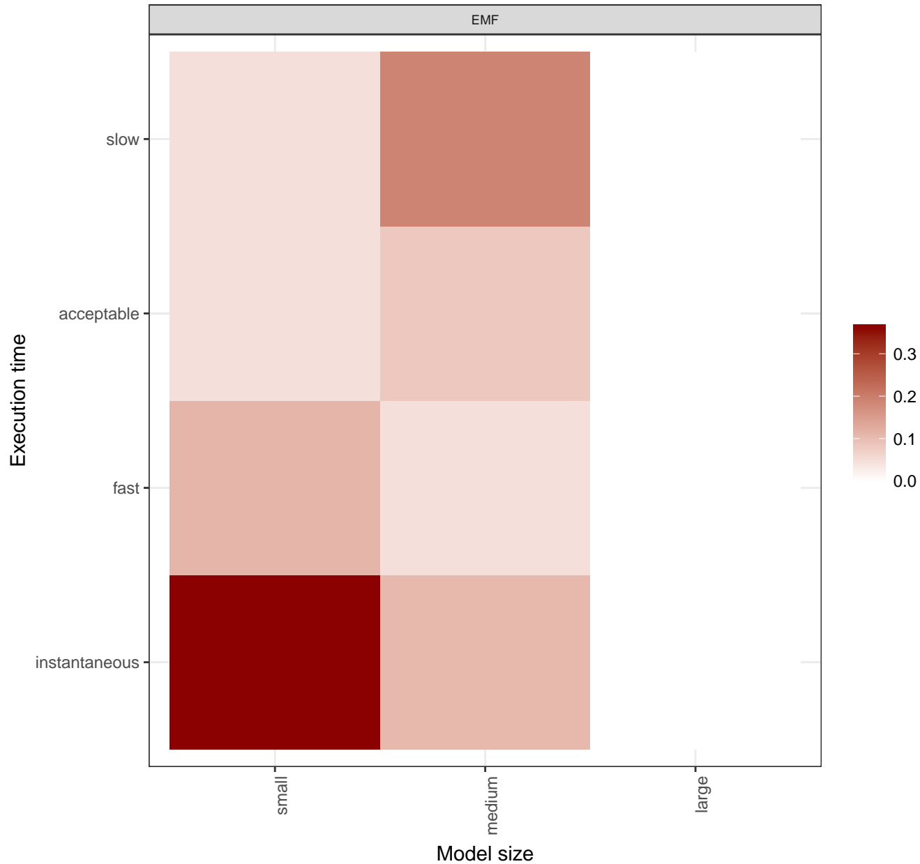
Comparison of performance by formats (total execution time)
